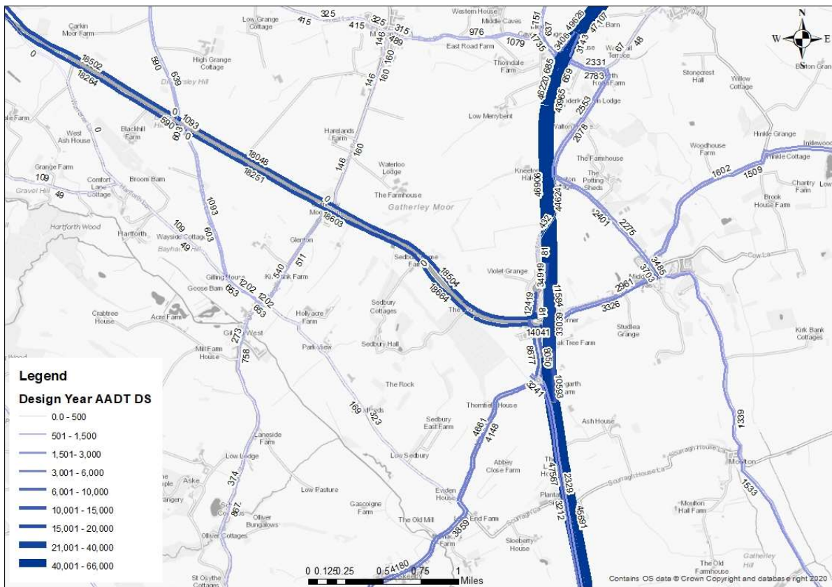
Figure 8-26: A1(M) Scotch Corner – Forecast Year Do Something Flows
