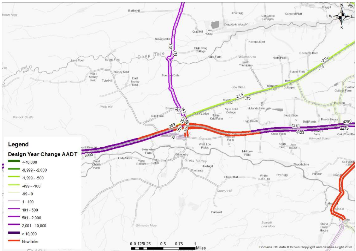
Figure 8-18: Bowes Bypass – Forecast Year Do Something Flows
