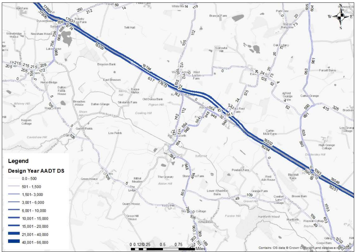
Figure 8-23: Stephen Bank to Carkin Moor – Forecast Year Do Something Flows
